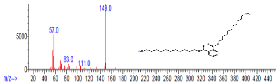
Fig. 1.1: Didodecyl phthalate
