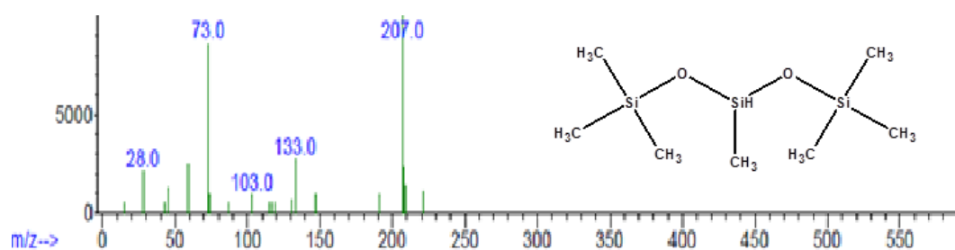
Fig. 1.6: 1,1,1,3,5,5,5-Heptamethyltrisiloxane
