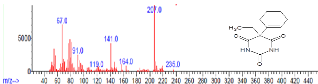
Fig. 1.4: Cyclobarbital
