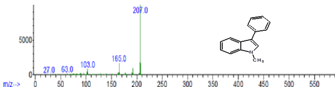
Fig. 1.13: 1-methyl-3-phenylindole
