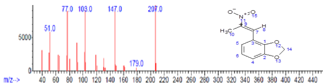
Fig. 1.5: Trans-2,3-methylenedioxy-b-methyl-b- nitrostyrene
