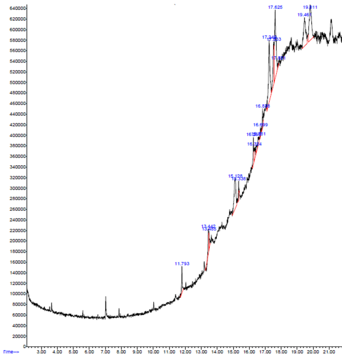
Fig. 1: GC-MS chromatogram of ethyl acetate extract of Cordia obliqua willd.
