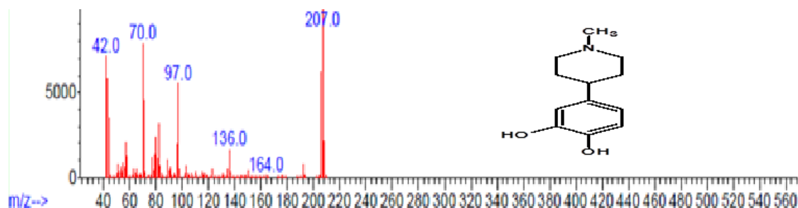
Fig. 1.8: Hexahydropyridine, 1-methyl-4-[4,5-dihydroxyphenyl]-
